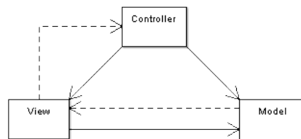
Fig. 1.2: Model-View-Controller diagram
